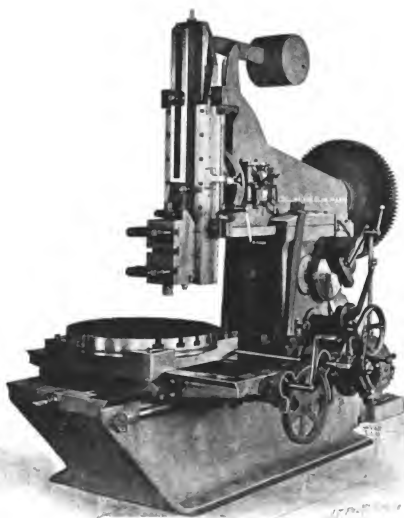
Fig. 5008. 16-Inch Traveling Head Slotter. T. C. Dill Machine Co., Inc.
